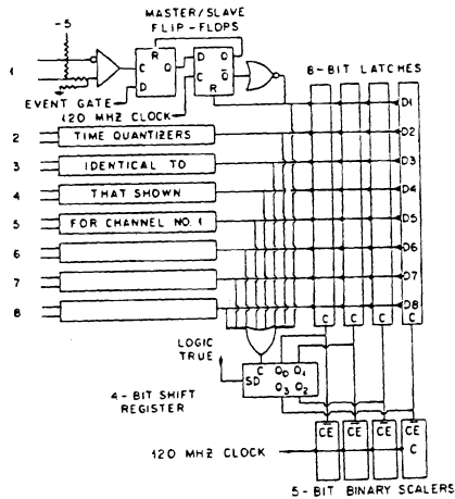
Fig. 5. Schematic Diagram of the Time Digitizer
